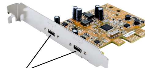
J3 & J4: 2x external USB 3.2 (Gen2) C-Port (screw lock)
