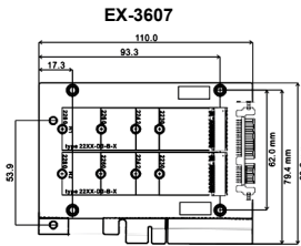
M.2 NFGG Modul B-Key / B+M-Key
